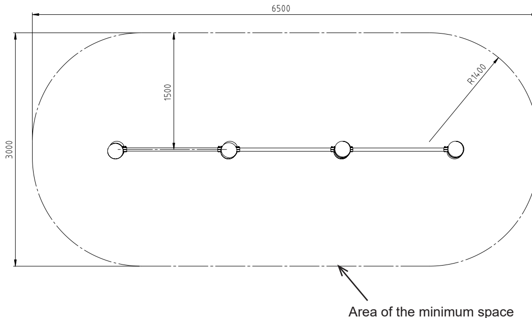
Diagram 4: Top view
